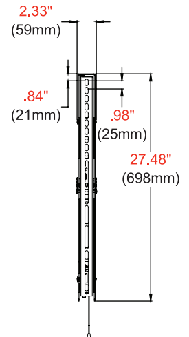
ADAPTER-DETAILS
